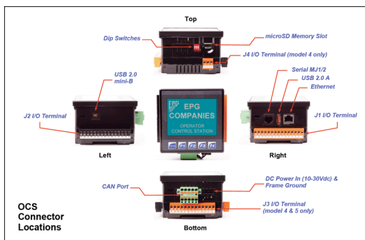
Above: OCS Connectors in detail.
