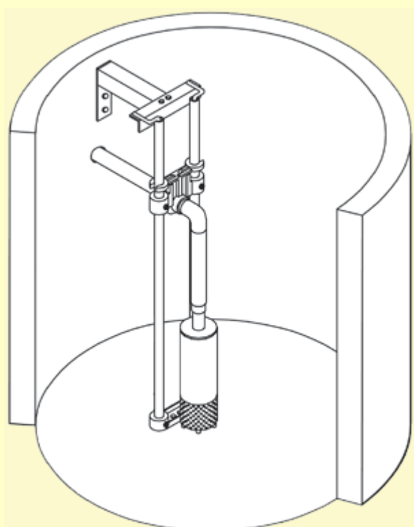
Common Guide Rail Installation For a Single SurePump™
